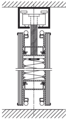
Ceiling/floor connection
